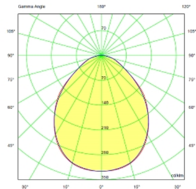
NFX-DN-8 Polar Diagram
